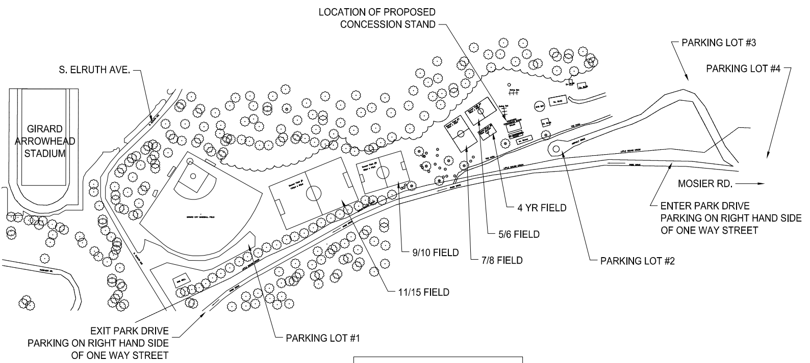
GIRARD / LIBERTY PARK FIELD AND PARKING LAYOUT
